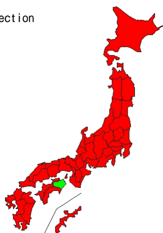
3493 cases A(H1)pdm09
